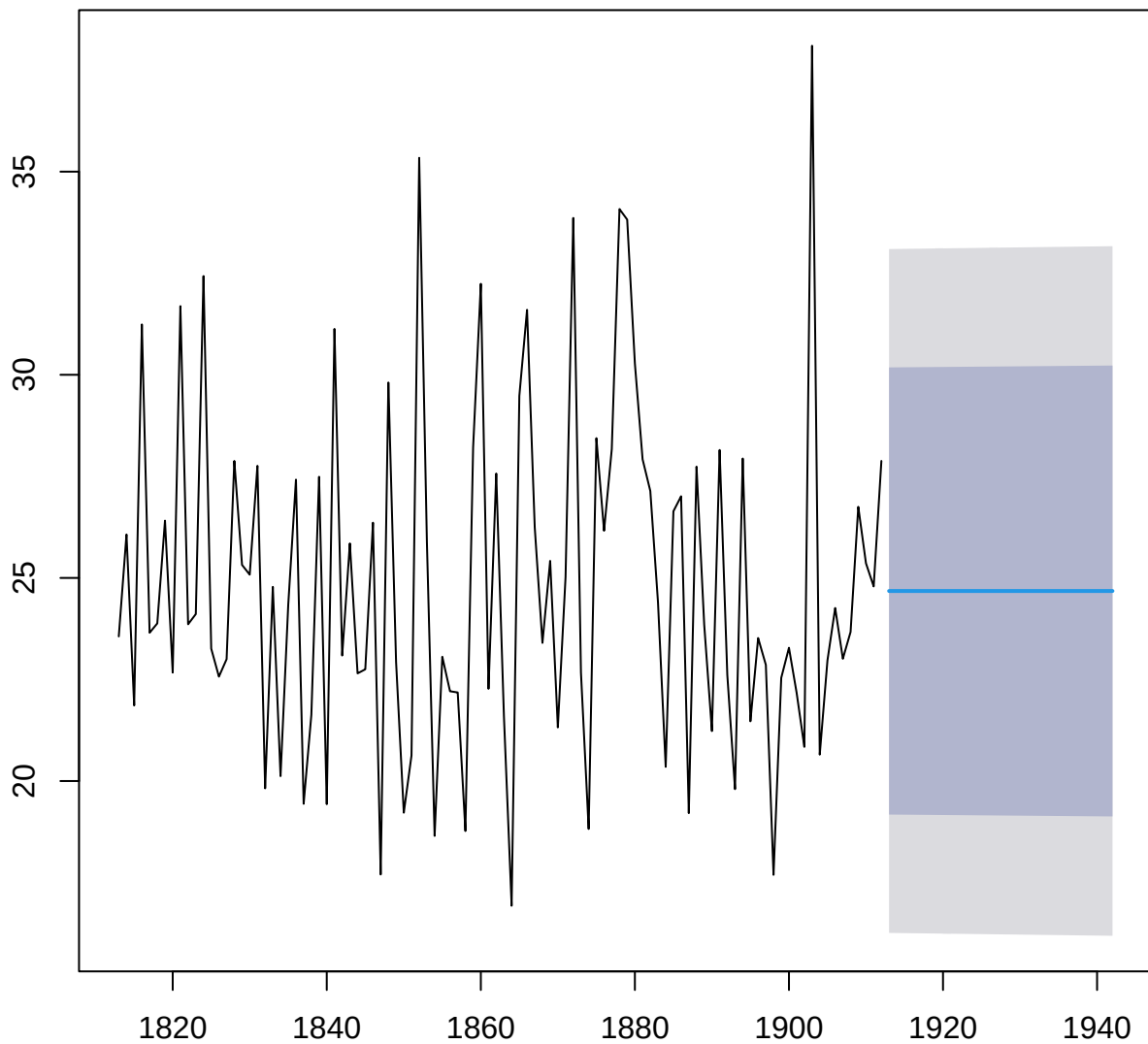
Forecasts from HoltWinters (h=30)
