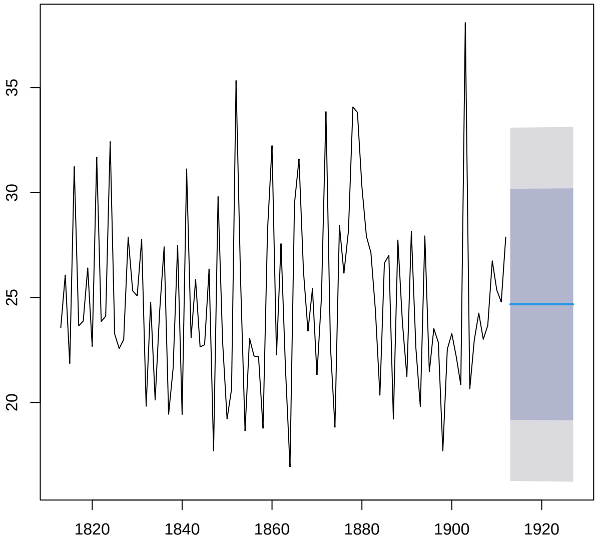
Forecasts from HoltWinters (h=15)
